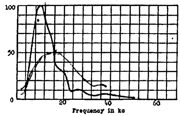
Fig. 3.111 Frequency function of broad- band pulse Shot No. 11 3400 km from ground zero
